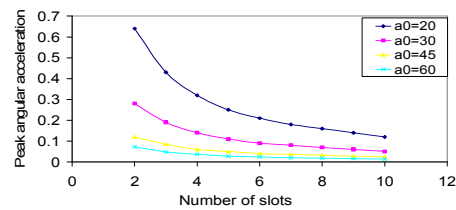
Fig.17. Peak angular acceleration for different number of slots for different \alpha_0 values
